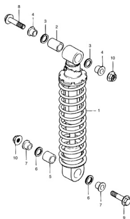
FIG.41 REAR SHOCK ABSORBER
