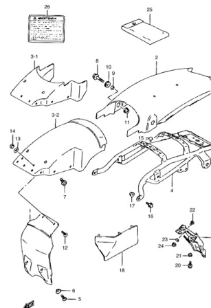
FIG.43B REAR FENDER
