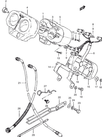
FIG.18 SPEEDOMETER/TACHOMETER
