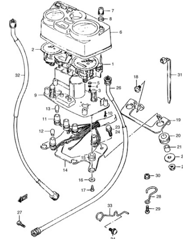
FIG.18B SPEEDOMETER
