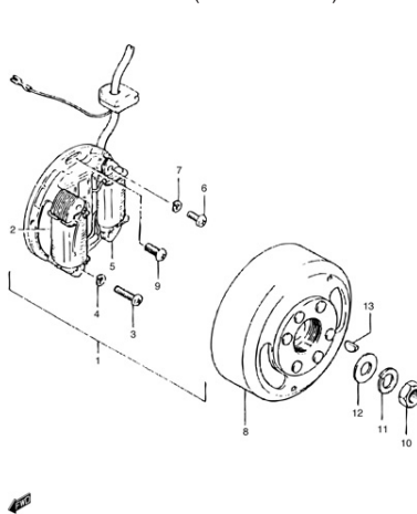
FIG.14 MAGNETO (model CR/CW)
