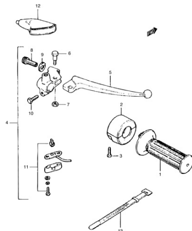
FIG.36 RIGHT HANDLE SWITCH
