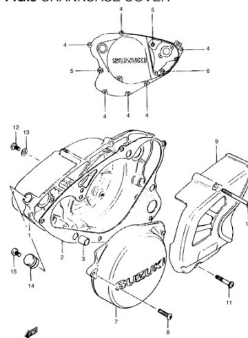
FIG.3 CRANKCASE COVER
