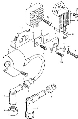
FIG.17 ELECTRICAL
