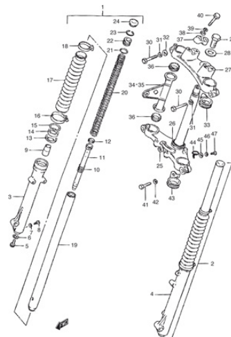
FIG.31A FRONT FORK
