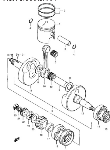
FIG.4 CRANKSHAFT
