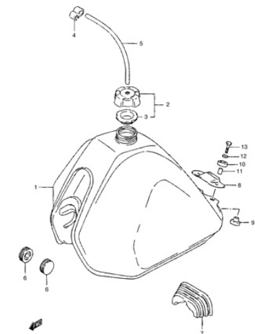
FIG.26A FUEL TANK
