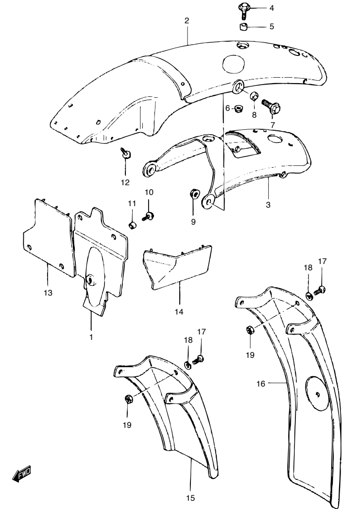
TS125ER_043 REAR FENDER
