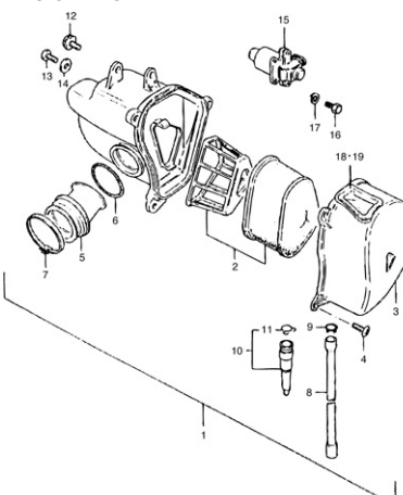
FIG.6 AIR CLEANER
