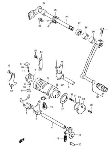
FIG.11 GEAR SHIFTING
