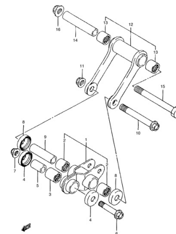
FIG.42A REAR CUSHION LEVER
