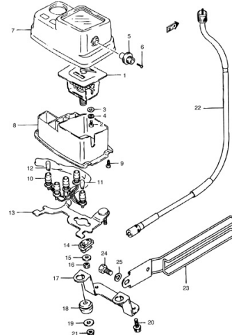
FIG.18A SPEEDOMETER
