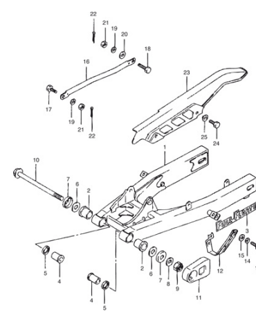
FIG.40A REAR SWINGING ARM
