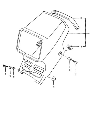
FIG.32B HEADLAMP COVER
