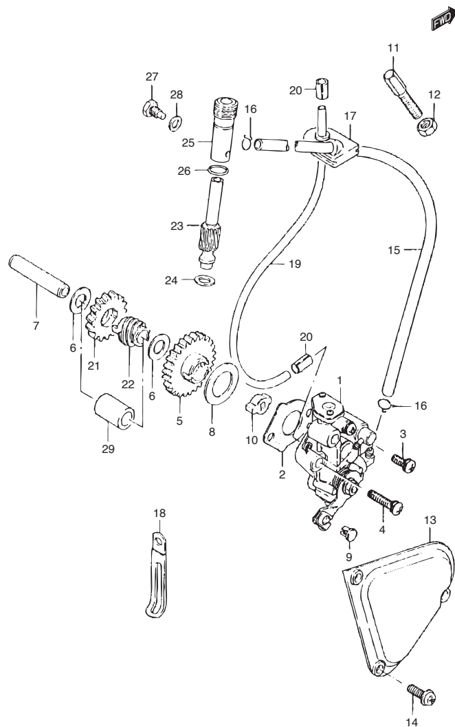
TS125ER_008 OIL PUMP
