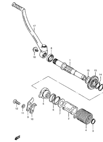
FIG.12 KICK STARTER
