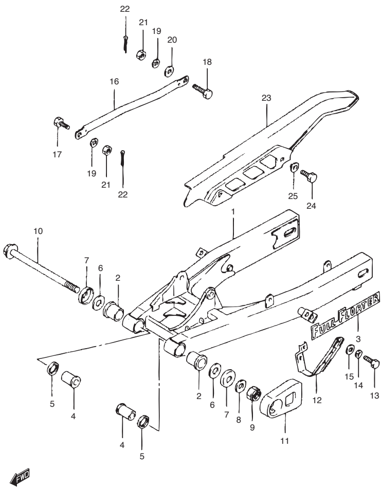
TS125ER_040A REAR SWINGING ARM
