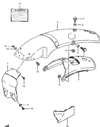
FIG.43A REAR FENDER
