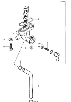
FIG.27 FUEL COCK
