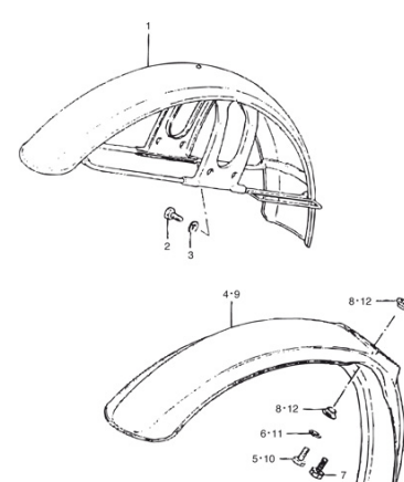
FIG.33 FRONT FENDER
