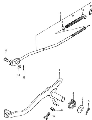
FIG.25 REAR BRAKE
