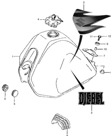
FIG.26B FUEL TANK
