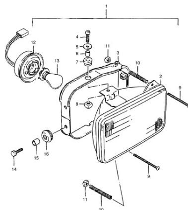
FIG.19A HEADLAMP
