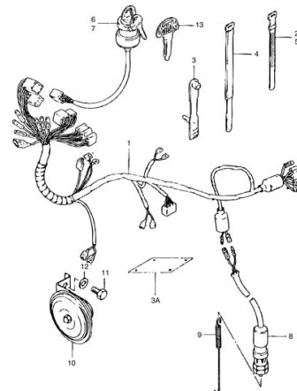
FIG.22 WIRING HARNESS
