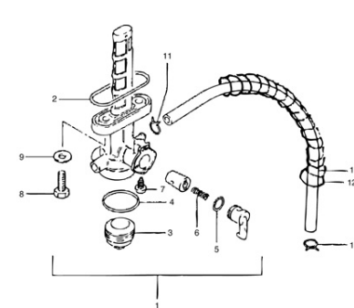
FIG.27A FUEL COCK
