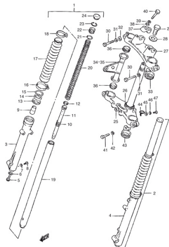
FIG.31 FRONT FORK
