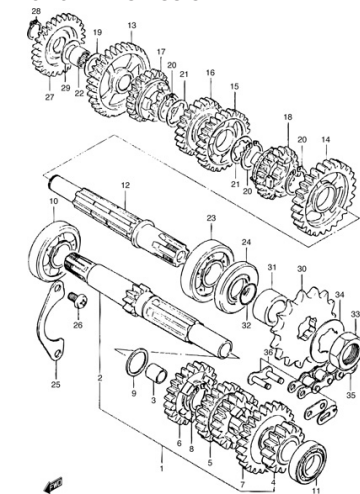
FIG.10 TRANSMISSION
