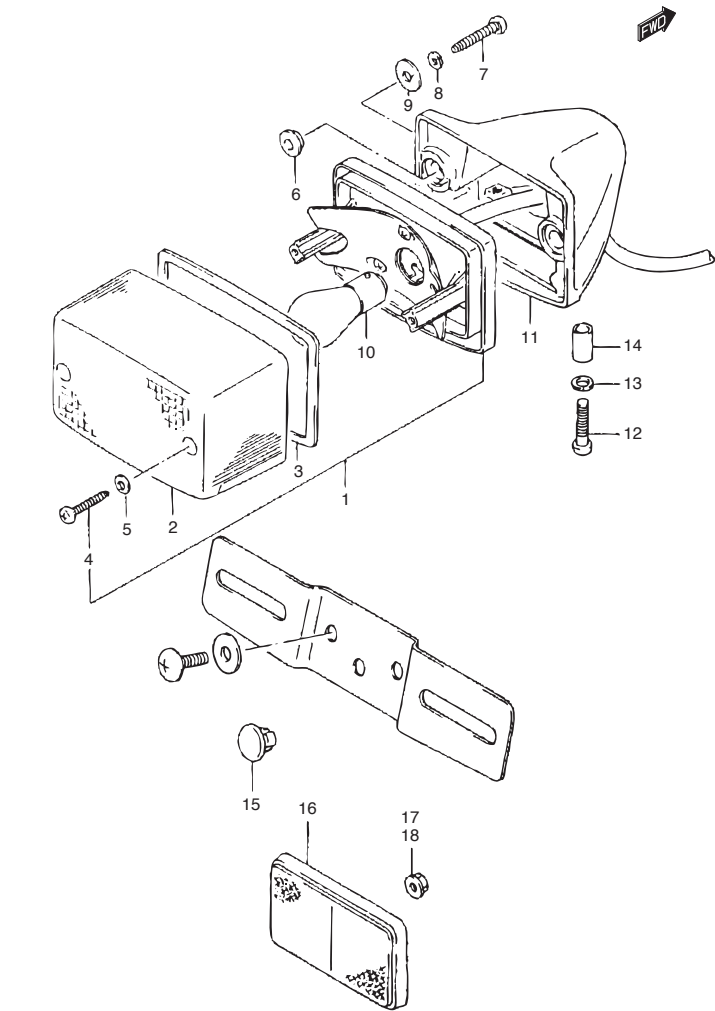
TS125ER_021A REAR COMBINATION LAMP
