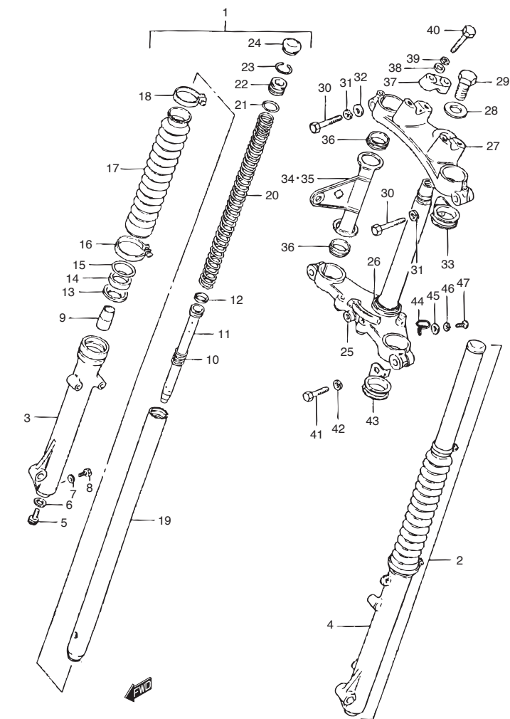
TS125ER_031A FRONT FORK
