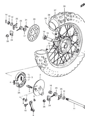
FIG.44 REAR WHEEL
