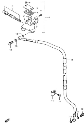
FIG.39 FRONT MASTER CYLINDER
