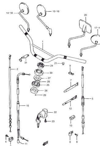
FIG.35 HANDLEBAR
