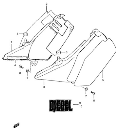
FIG.30A FRAME COVER
