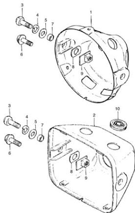
FIG.32 HEADLAMP HOUSING
