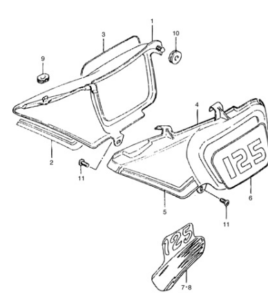
FIG.30 FRAME COVER
