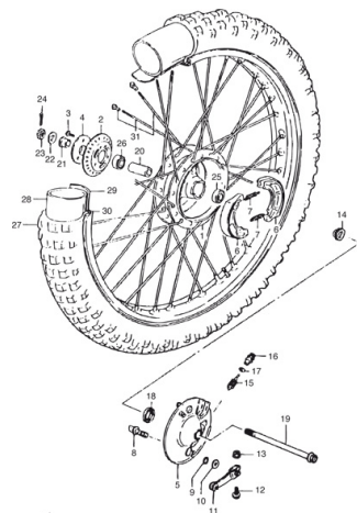
FIG.34 FRONT WHEEL
