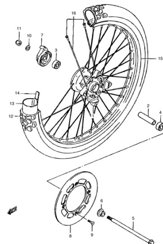
FIG.34A FRONT WHEEL
