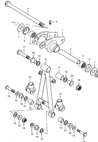
FIG.42 REAR CUSHION LEVER
