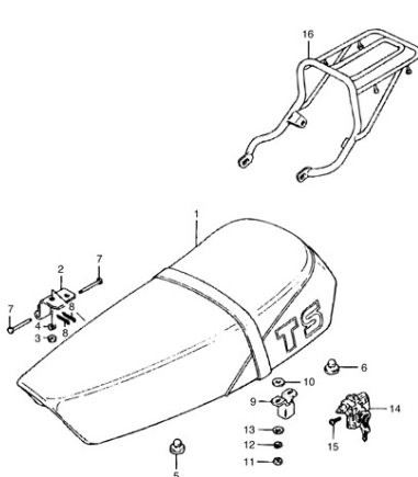
FIG.29 SEAT
