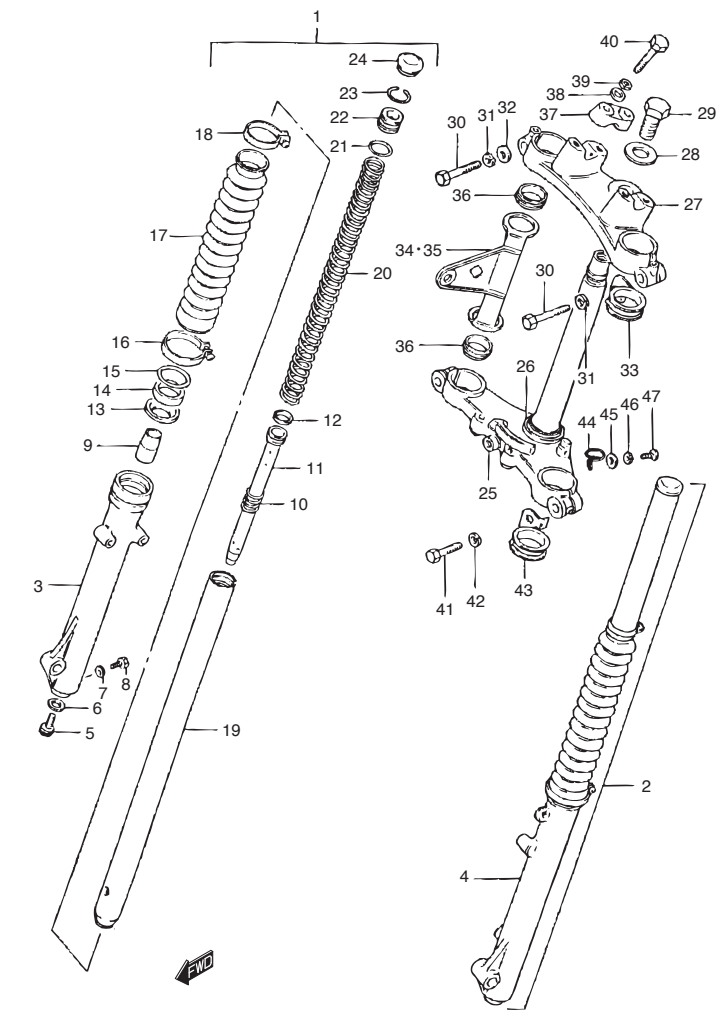
TS125ER_031 FRONT FORK
