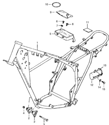
FIG.23 FRAME
