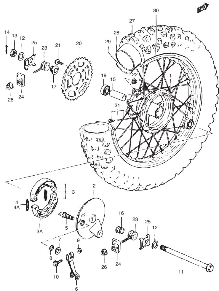
TS125ER_044 REAR WHEEL
