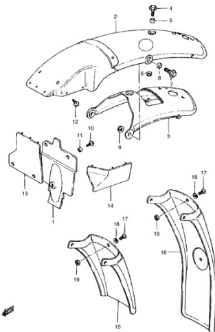
FIG.43 REAR FENDER
