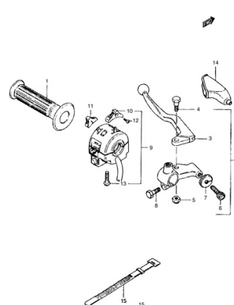
FIG.37 LEFT HANDLE SWITCH
