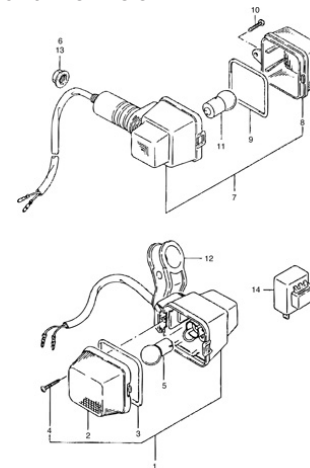
FIG.20A TURN SIGNAL LAMP
