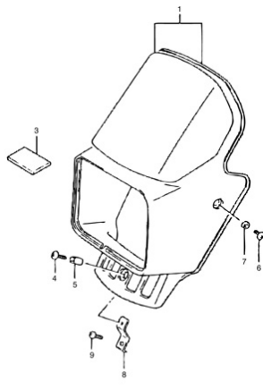
FIG.32A HEADLAMP COVER
