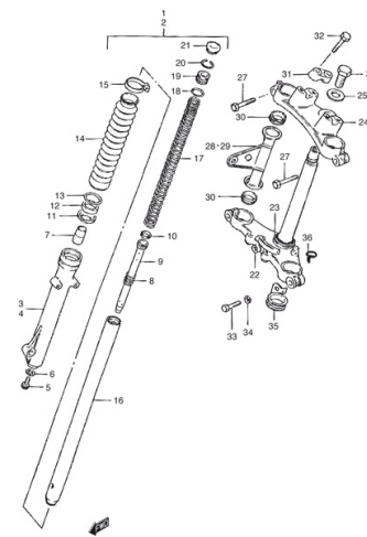
FIG.31B FRONT FORK
