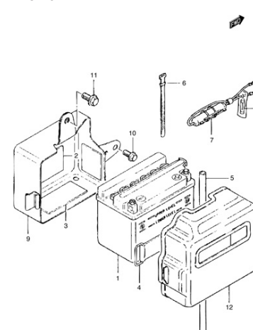
FIG.16 BATTERY
