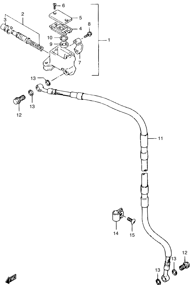
TS125ER_039 FRONT MASTER CYLINDER
