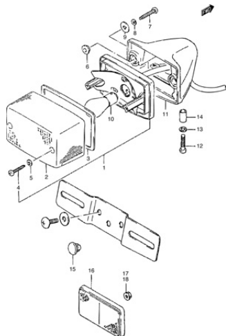
FIG.21A REAR COMBINATION LAMP
