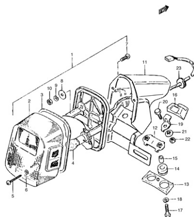
FIG.21 REAR COMBINATION LAMP
