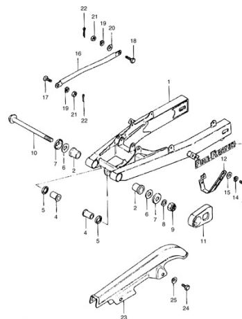
FIG.40 REAR SWINGING ARM
