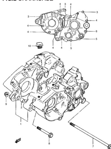
FIG.2 CRANKCASE
