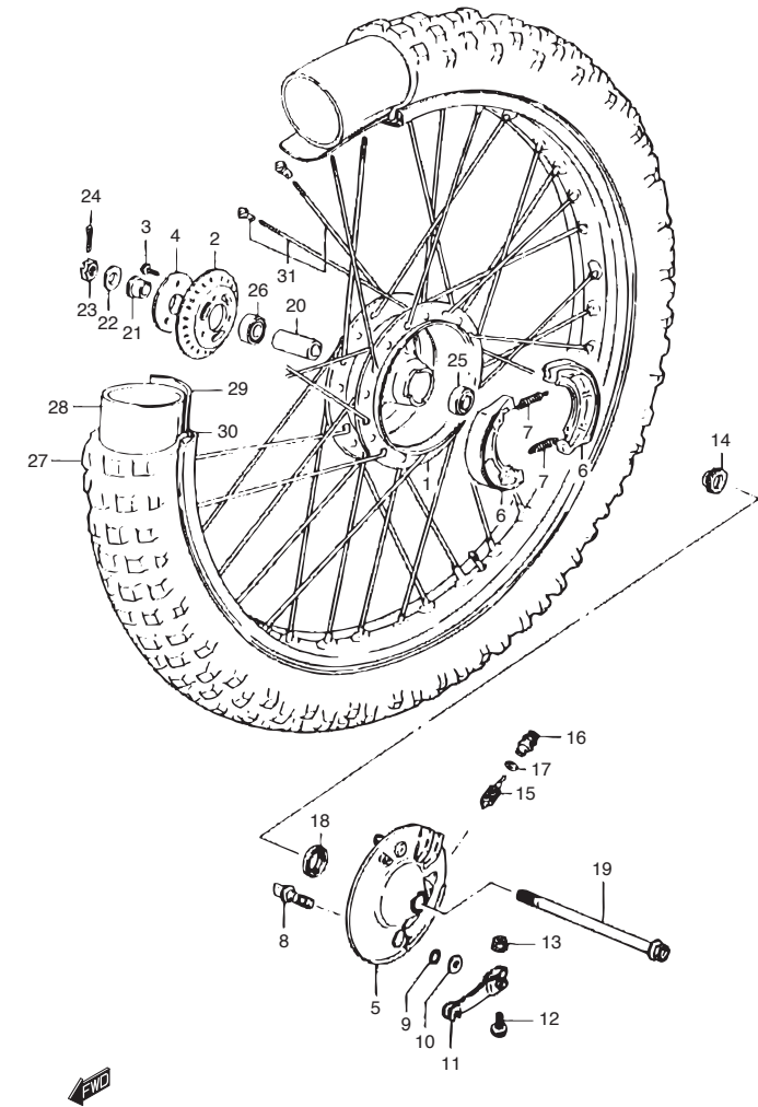
TS125ER_034 FRONT WHEEL
