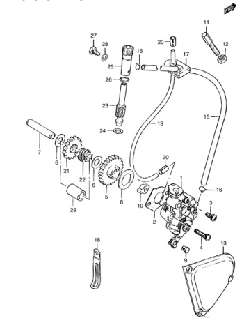
FIG.8 OIL PUMP
