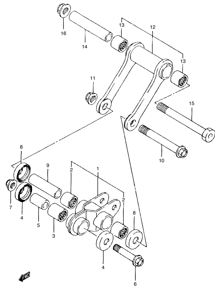
TS125ER_042A REAR CUSHION LEVER
