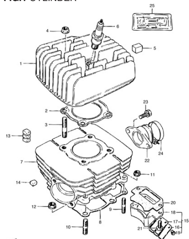
FIG.1 CYLINDER
