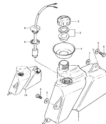
FIG.28 OIL TANK
