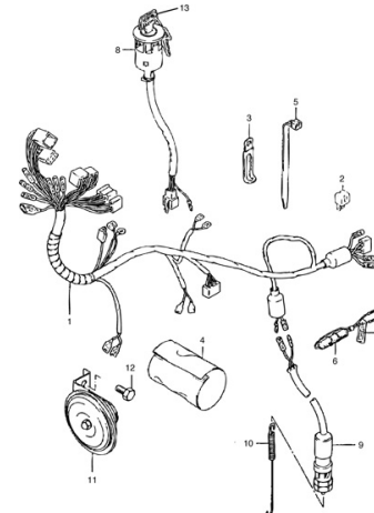
FIG.22A WIRING HARNESS
