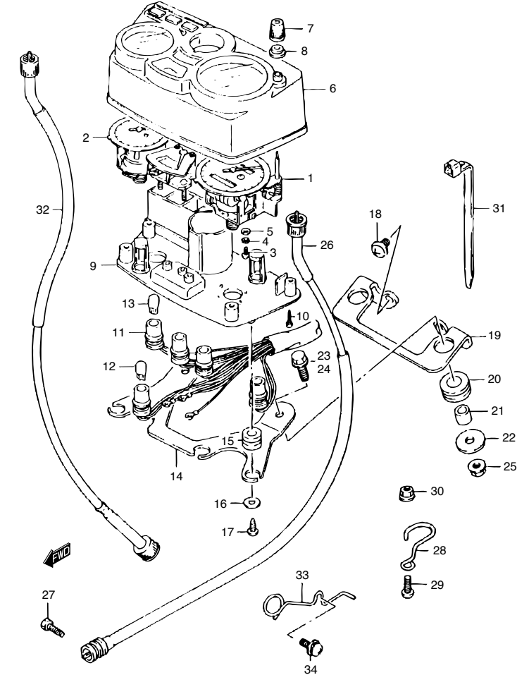
TS125ER_018B SPEEDOMETER
