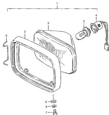
FIG.19 HEADLAMP
