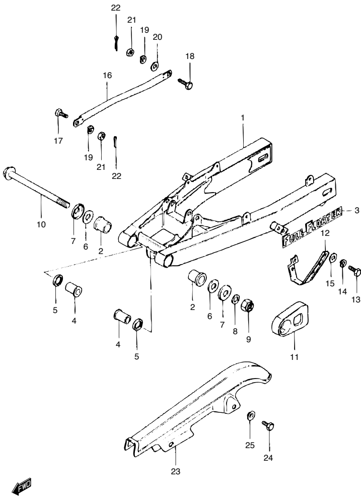
TS125ER_040 REAR SWINGING ARM
