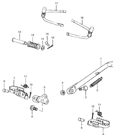
FIG.24 STAND - FOOTREST
