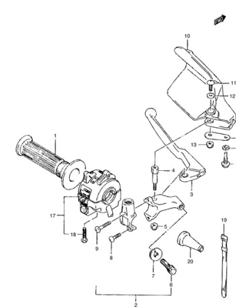
FIG.37A LEFT HANDLE SWITCH
