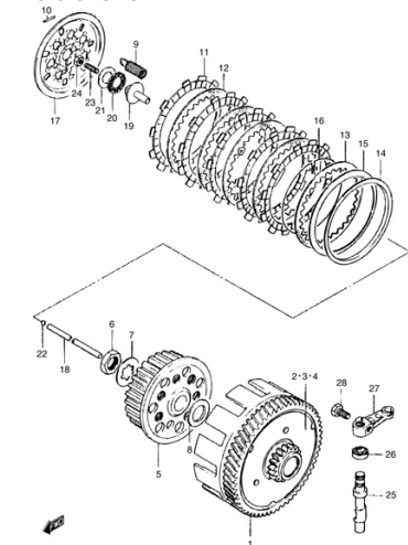
FIG.9 CLUTCH
