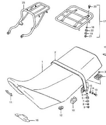
FIG.29A SEAT
