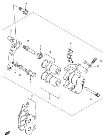
FIG.38 FRONT CALIPER
