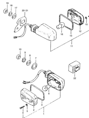
FIG.20 TURN SIGNAL LAMP
